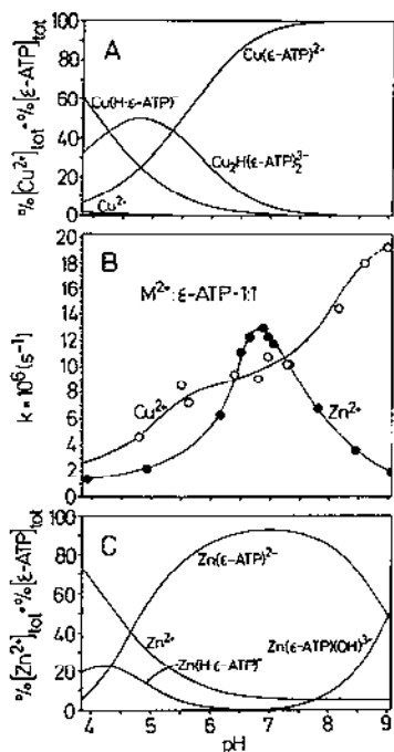
Fig. 30. Comparison of the variation of (B) the Cu^{2+} -promoted (O) and Zn^{2+} -promoted (●) dephosphorylation of \epsilon -ATP (each 10^{-3} M) in aqueous solution at 50^\circ C as a function of pH ( I = 0.1 M, NaClO_4 ; cf. Fig. 27), with the effect of pH at 25^\circ C ( I = 0.1 M, NaNO_3 ) on the concentration of the species present in an aqueous solution of Cu^{2+} (A) or Zn^{2+} (C) and \epsilon -ATP (each 10^{-3} M). These results were computed with the constants listed in Table I in ref. 86, and they are given as the percentage of the total M^{2+} present (equal to total \epsilon -ATP); for the formation of Cu(\epsilon-ATP)(OH)^{3-} holds probably pK_{Cu(\epsilon-ATP)(H_2O)}^H > 8.5 [86]. (Reproduced from Fig. 7 in ref. 86 (Inorganic Chemistry, 1986) with permission of the American Chemical Society.)
