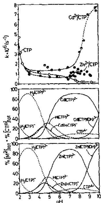
Fig. 8. Comparison of the variation (upper part) of the \text{Cd}^{2+} -promoted (●) [65] and \text{Zn}^{2+} -promoted (●) [66] dephosphorylation of CTP (alone: ○) [69] in aqueous solution at 50^\circ\text{C} , characterized by first-order rate constants k ( \text{s}^{-1} ), as a function of pH (each reactant, when present, was 10^{-3} M; I = 0.1 M, \text{NaClO}_4 ; the broken line portions indicate uncertainty due to precipitation) with the effect (lower parts) of pH at 25^\circ\text{C} ( I = 0.1 M, \text{Na}^+ \text{ClO}_4^- / \text{NO}_3^- ) on the concentration of the species present in an aqueous solution of CTP and \text{Cd}^{2+} or \text{Zn}^{2+} (each 10^{-3} M); these results are given as the percentage of the total \text{M}^{2+} present (equal to total CTP); the broken lines refer to the free CTP species and the solid lines to the CTP complexes. The results of the middle and lower parts were computed with the following equilibrium constants: \text{p}K_{\text{H}_3(\text{CTP})}^{\text{H}} \approx 1.6 ( \approx \text{p}K_{\text{H}_3(\text{ATP})}^{\text{H}} [72]), \text{p}K_{\text{H}_2(\text{CTP})}^{\text{H}} = 4.55 \pm 0.03 , \text{p}K_{\text{H}(\text{CTP})}^{\text{H}} = 6.55 \pm 0.02 , \log K_{\text{Cd}(\text{H} \cdot \text{CTP})}^{\text{Cd}} = 3.15 \pm 0.06 , \log K_{\text{Zn}(\text{H} \cdot \text{CTP})}^{\text{Zn}} = 3.05 \pm 0.07 , \log K_{\text{Cd}(\text{CTP})}^{\text{Cd}} = 5.05 \pm 0.04 , \log K_{\text{Zn}(\text{CTP})}^{\text{Zn}} = 5.03 \pm 0.05 (all values from ref. 61), \text{p}K_{\text{Cd}(\text{CTP})(\text{H}_2\text{O})}^{\text{H}} = 10.0 [88], \text{p}K_{\text{Zn}(\text{CTP})(\text{H}_2\text{O})}^{\text{H}} = 8.79 \pm 0.05 [73]. The diprotonated \text{M}(\text{H}_2 \cdot \text{CTP}) complexes were ignored in the calculations as the appropriate constants are unknown; however, such species would probably exist only below pH 3.
