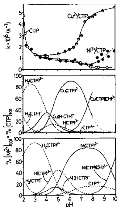
Fig. 7. Comparison of the variation (upper part) of the Cu^{2+} -promoted ( \bullet ) [69] and Ni^{2+} -promoted ( \bullet ) [66] dephosphorylation of CTP (alone, \circ ) [69] in aqueous solution at 50^\circ C , characterized by first-order rate constants k ( s^{-1} ), as a function of pH (each reactant when present was 10^{-3} M ; I = 0.1 M , NaClO_4 ; the broken line portion indicates uncertainty due to precipitation) with the effect (lower parts) of pH at 25^\circ C ( I = 0.1 M , Na^+ ClO_4^- / NO_3^- ) on the concentration of the species present in an aqueous solution of CTP and Cu^{2+} or Ni^{2+} (each 10^{-3} M ); these results are given as the percentage of the total M^{2+} present (equal to total CTP); the broken lines refer to the free CTP species and the solid lines to the CTP complexes. The results of the middle and lower parts were computed with the following equilibrium constants: pK_{H_3(CTP)}^H \approx 1.6 ( \approx pK_{H_3(ATP)}^H [72]), pK_{H_2(CTP)}^H = 4.55 \pm 0.03 , pK_{H(CTP)}^H = 6.55 \pm 0.02 , \log K_{Cu(H \cdot CTP)}^{Cu} = 3.80 \pm 0.06 , \log K_{Ni(H \cdot CTP)}^{Ni} = 2.70 \pm 0.25 , \log K_{Cu(CTP)}^{Cu} = 6.03 \pm 0.03 , \log K_{Ni(CTP)}^{Ni} = 4.52 \pm 0.02 (all values from ref. 61), pK_{Cu(CTP)(H_2O)}^H = 7.6 [73,89] (this value describes the situation well in the pH range up to 8, possibly even 9, then matters may become more complicated and therefore at pH > 8 the lines are dotted; this conclusion is made in analogy to the Cu^{2+}/ATP system, cf. refs. 55 and 63), pK_{Ni(CTP)(H_2O)}^H = 9.58 \pm 0.15 [73]. The diprotonated M(H_2 \cdot CTP) complexes were ignored in the calculations as the appropriate constants are unknown; however, such species would probably exist only below pH 3.
