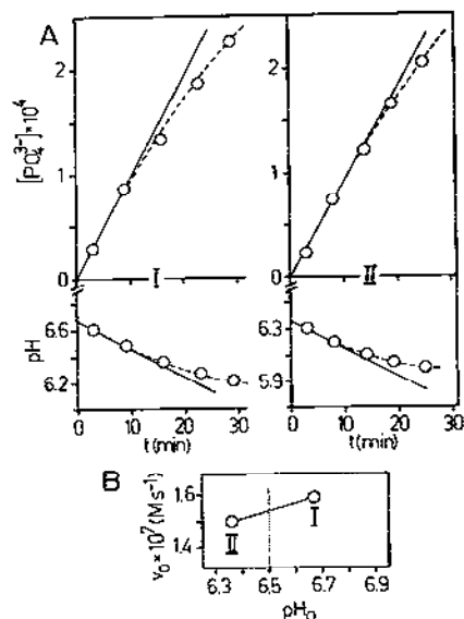
Fig. 3. Determination of the initial rate v_0 (M s ^{-1} ) and the corresponding initial pH, pH_0 (A), and the interpolation (B) for v_0 at pH_0 6.50. A, Cu^{2+} -promoted dephosphorylation of ATP in aqueous solution; [ATP]_{tot(t=0)} = 0.9 \times 10^{-3} M, [Cu^{2+}]_{tot} = 1.1 \times 10^{-3} M (there is a printing error in the concentrations given in ref. 64); I = 0.1 M, NaClO_4 ; 50^\circ C . Initial rate for case I and extrapolation to t = 0 : v_0 = d[PO_4^{3-}]/dt = 1.91 \times 10^{-4}/(20 \times 60) = 1.59 \times 10^{-7} M s ^{-1} ( pH_0 6.67). For case II: v_0 = 1.80 \times 10^{-4}/(20 \times 60) = 1.50 \times 10^{-7} M s ^{-1} ( pH_0 6.36). B, interpolation from the above results at pH_0 6.50 gives v_0 = 1.54 \times 10^{-7} M s ^{-1} ; this value corresponds to the top point of the experimental series at pH_0 6.50 shown in Fig. 15B (vide infra in Section E(ii)). (Partial reproduction from Fig. 1 in ref. 64 (J. Am. Chem. Soc., 1976) with permission of the American Chemical Society.)
