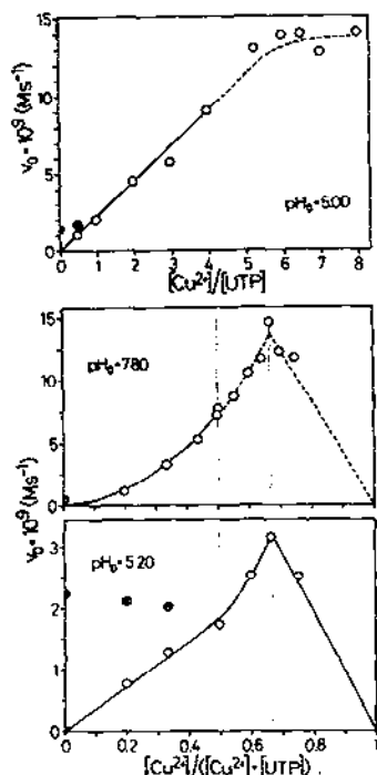
Fig. 10. Upper part: Dependence of the initial rate v_0 (M s -1 ) for the Cu 2+ -promoted dephosphorylation of UTP in water on the ratio [Cu^{2+}]/[UTP] with [UTP]_{tot} = 10^{-3} M at pH 0 5.00. Lower parts: Job's series for the aqueous Cu 2+ /UTP system at pH 0 7.80 and 5.20 at [Cu^{2+}]_{tot} + [UTP]_{tot} = \text{constant} = 2 \times 10^{-3} M. The vertical dotted lines give the positions of the ratios Cu 2+ : UTP = 1 : 1 or 2 : 1 (see text). For all three parts, I = 0.1 M, NaClO 4 ; 50°C. The measured points (⊗) were corrected for the dephosphorylation rate of uncomplexed UTP by assuming that the 1 : 1 complex, Cu(UTP) 2- , is completely formed. The broken line portions indicate uncertainty due to precipitation. This figure is a combination of the data given in Figs. S5 and S6 in ref. 71.
