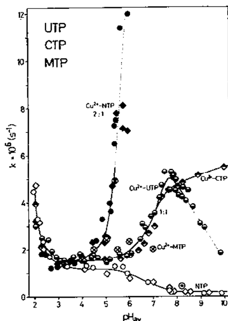
Fig. 6. First-order rate constants, k ( \text{s}^{-1} ), for the dephosphorylation of UTP ( \circ , \ominus , \bullet ) and CTP ( \diamond , \diamond , \blacklozenge ) in aqueous solution as a function of pH: NTP alone ( \circ , \diamond ), \text{Cu}^{2+}/\text{NTP} (1:1) ( \ominus , \diamond ), and \text{Cu}^{2+}/\text{NTP} (2:1) ( \bullet , \blacklozenge ); [\text{NTP}]_{\text{tot}} = 10^{-3} M; I = 0.1 M, \text{NaClO}_4 ; 50^\circ\text{C} . The dotted line portions indicate uncertainty due to precipitation. For further comparison the corresponding data for methyltriphosphate [34] are also shown: MTP ( \circ ), \text{Cu}^{2+}/\text{MTP} (1:1) ( \ominus ), and \text{Cu}^{2+}/\text{MTP} (2:1) ( \bullet ); [\text{MTP}]_{\text{tot}} = 10^{-3} M; 50^\circ\text{C} . (Reproduced from Fig. 3 in ref. 71 (Eur. J. Biochem., 1983) with permission.)
