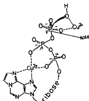
Fig. 31. Probable structure of the reactive \text{Cu}_2(\epsilon\text{-ATP})(\text{OH})^- complex formed during the \text{Cu}^{2+} -promoted dephosphorylation of \epsilon -ATP (see text).
