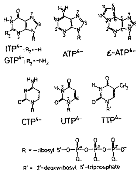
Fig. 1. Structures of several nucleoside 5'-triphosphates ( \text{NTP}^{4-} ), together with the labeling system for the triphosphate chain. It should be noted that the phosphate groups in the NTPs are labeled \alpha , \beta , and \gamma , where \gamma refers to the terminal phosphate residue. To facilitate comparisons (see Section H) between the \epsilon -adenine and the adenine residues in \epsilon\text{-ATP}^{4-} (equal to 1,N^6\text{-etheno-ATP}^{4-} ) and \text{ATP}^{4-} respectively, the conventional atom numbering for adenines is adapted [28]. Obviously, the analogous nucleoside 5'-monophosphates ( \text{NMP}^{2-} ) have the corresponding structures with only a single phosphate group.
