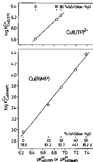
Fig. 33. Relationships between \log K_{\text{Cu}}^{\text{Cu(UTP)}} and \text{pK}_{\text{H}}^{\text{H(UTP)}} , and \log K_{\text{Cu}}^{\text{Cu(RiMP)}} and \text{pK}_{\text{H}}^{\text{H(RiMP)}} for the \text{Cu(UTP)}^{2-} and \text{Cu(RiMP)} complexes respectively as they result from the addition of increasing amounts of 1,4-dioxane to the aqueous solutions of the components ( I = 0.1 \text{ M} , \text{NaNO}_3 ; 25^\circ \text{C} ). The plotted equilibrium constants are for uridine 5'-triphosphate (UTP) and D-ribose 5'-monophosphate (RiMP) from ref. 15 and ref. 161 respectively. The various percentages of the dioxane-water mixtures (v/v) which correspond to the data points are inserted into the figure; also inserted are the corresponding dielectric constants ( \epsilon ); these latter values are interpolated from the data given in ref. 162.
