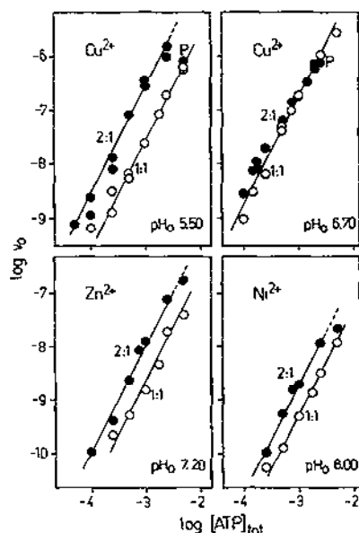
Fig. 17. Relationship between the initial dephosphorylation rates v_0 ( M s^{-1} ) of ATP and the total concentrations of M^{2+} and ATP in aqueous solution for different metal ions at various values of pH_0 . Dependence of \log v_0 on \log [ATP]_{tot} = \log [M^{2+}]_{tot} (O) or \log [ATP]_{tot} = \log (1/2[M^{2+}]_{tot}) (●); I = 0.1 M , NaClO_4 ; 50^\circ C . The solid lines are drawn with the slope m = 2 (see text); the broken line portions indicate uncertainty due to precipitation. In the experiments labeled P, precipitation was also observed. (Reproduced from Fig. 9 in ref. 64 (J. Am. Chem. Soc., 1976) with permission of the American Chemical Society.)
